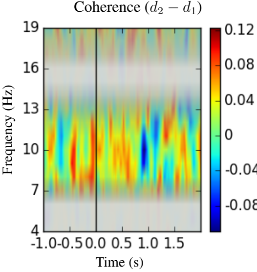
Figure 3: A time-frequency depiction of the mean coherence in the depth = 1 condition subtracted from the mean coherence in the depth = 2 condition in development data. An overlay conveys the variance of different frequency bands. Faded regions have higher variance than clearer regions.
